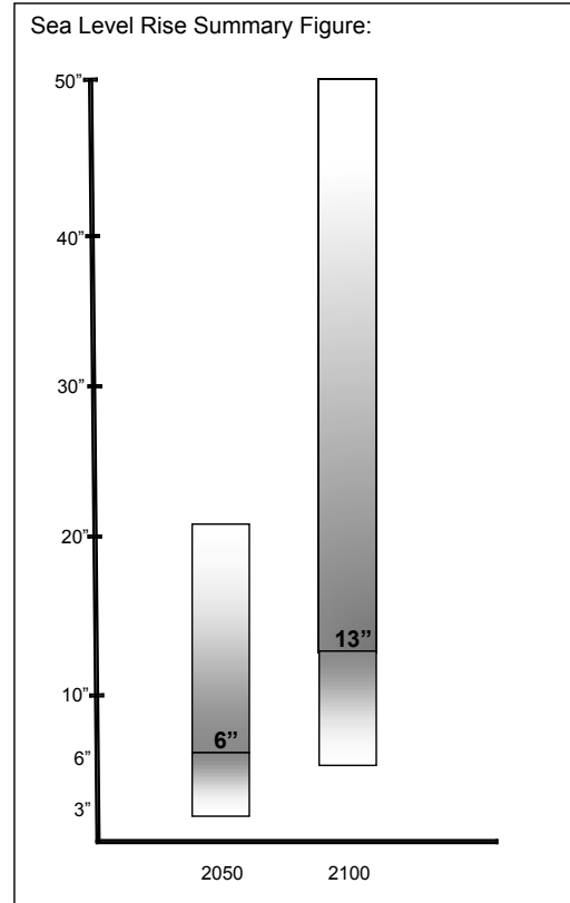
Projected sea level rise in Washington's waters relative to 1980-99, in inches. Shading roughly indicates likelihood.
