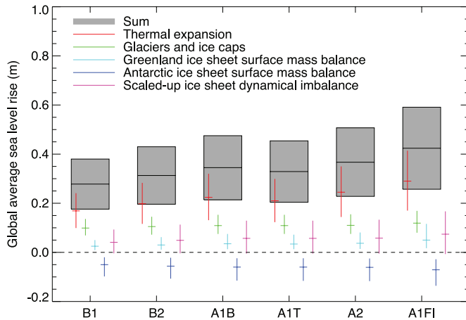
Figure 3. Projections and uncertainties (5 to 95% ranges) of global average sea level rise and its components in 2090 to 2099 (relative to 1980 to 1999) for the six SRES marker scenarios. The projected sea level rise assumes that the part of the present-day ice sheet mass imbalance that is due to recent ice flow acceleration will persist unchanged. It does not include the contribution shown from scaled-up ice sheet discharge, which is an alternative possibility. It is also possible that the present imbalance might be transient, in which case the projected sea level rise is reduced by 0.02 m. It must be emphasized that we cannot assess the likelihood of any of these three alternatives, which are presented as illustrative. The state of understanding prevents a best estimate from being made. From IPCC (2007).
