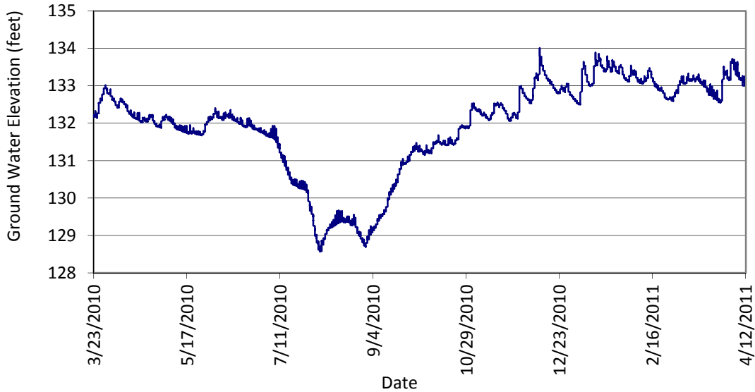
Figure 4. Shallow groundwater elevation time series data. Bertrand Creek Subbasin- Well BAE 184. T41N, R2E, Section 36. Ground surface elevation approximately 140 feet.
