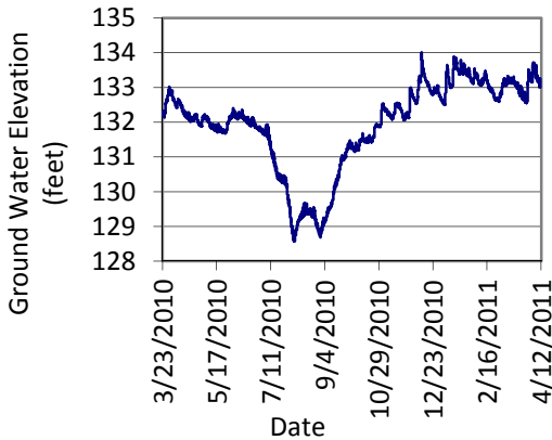
Figure 5. Shallow groundwater hydrograph. Bertrand Creek Subbasin- Well BAE 184. T41N, R2E, Section 36. Ground surface elevation approximately 140 feet.
