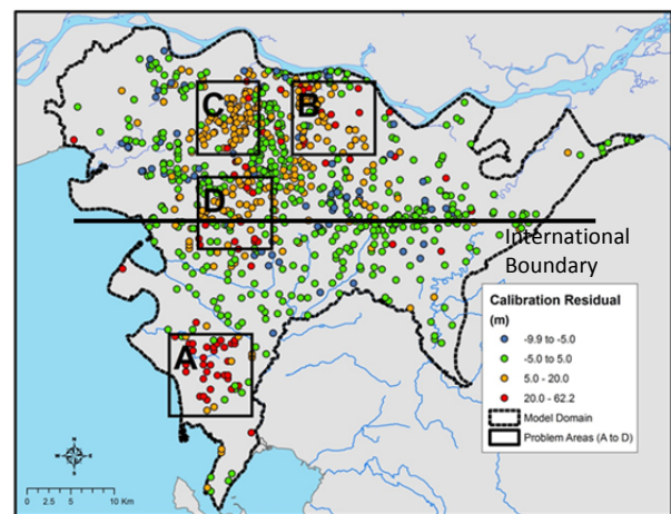
Figure 11. FE Flow groundwater model extent and calibration results (Simpson, 2012).
